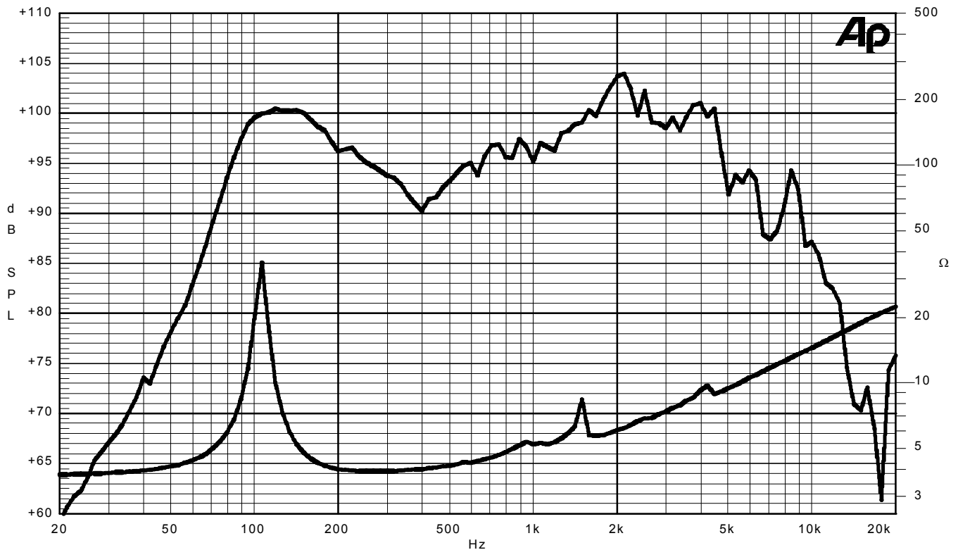
Frequency Response on IEC Baffle (DIN 45575) @ 1 W, 1 m -
